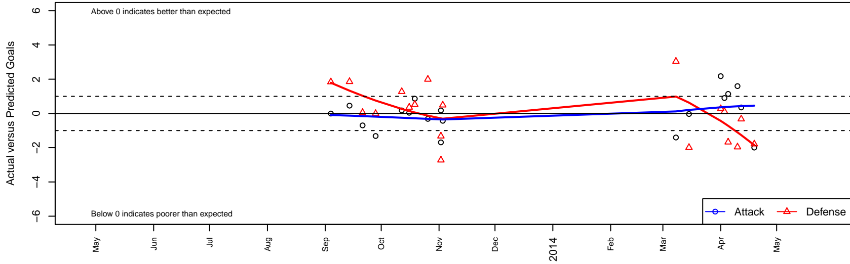
Idaho Arsenal United Hurricanes G01 Dots are actual minus expected GF (blue circles) and GA (red triangles). Blue line is smoothed change in attack strength. Red is smoothed change in defense strength.
